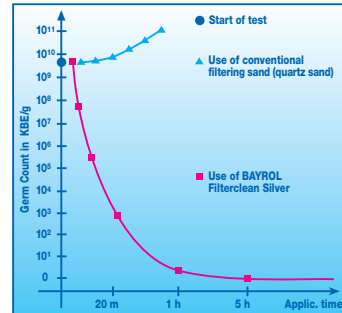
Germ degradation versus germ growth with circulating pump switched off (using a test model)
